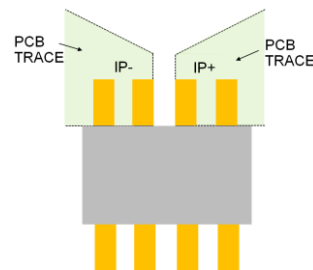
Figure 13: Recommended Trace Layout on the Input Pins
