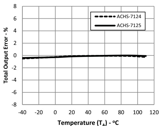
Figure 6: Total Output Error at I_{P(MAX)} vs. Temperature
