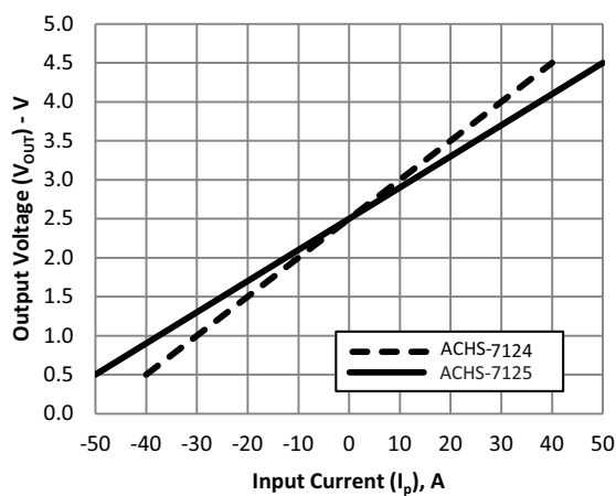
Figure 4: Output Voltage vs. Input Current
